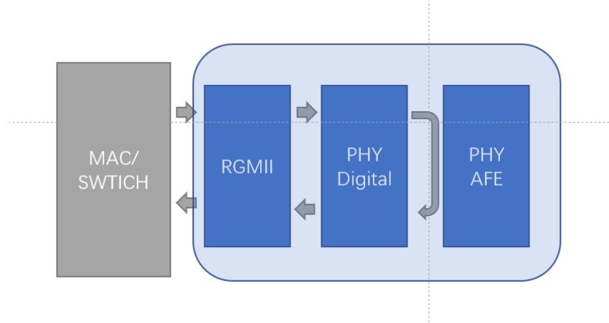
Figure . digital loopback
